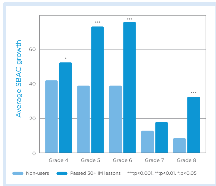
Figure 1. SBAC Math Score Growth
